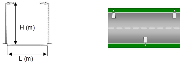
Figura 3: Posteamto Bilateral Alternada
